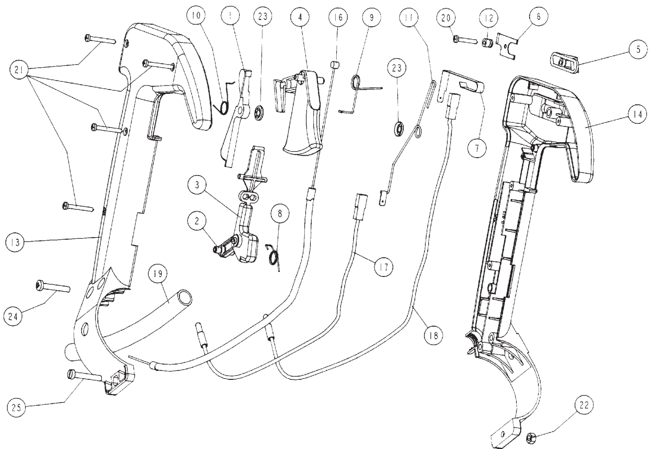
FIG.03 MANOPLA
